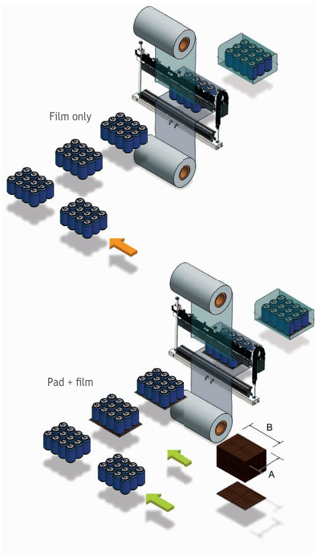
Pad insertion device
